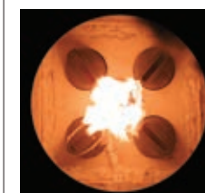
Ordinary Flame Region (Air ratio 3.0)
